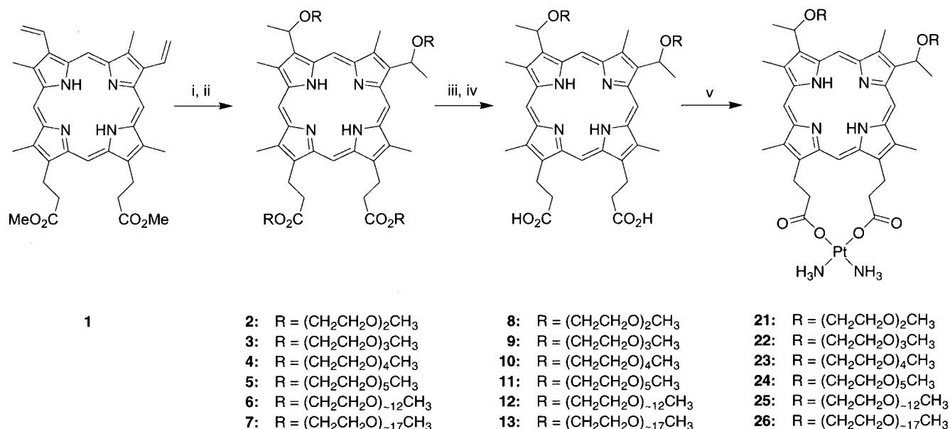
Scheme 1 a
